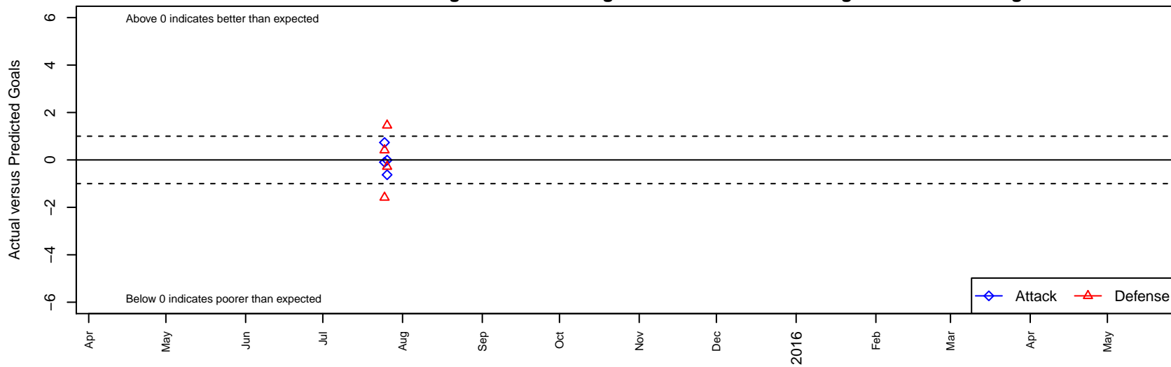
San Diego United Black G98 Dots are actual minus expected GF (blue circles) and GA (red triangles). Blue line is smoothed change in attack strength. Red is smoothed change in defense strength.
